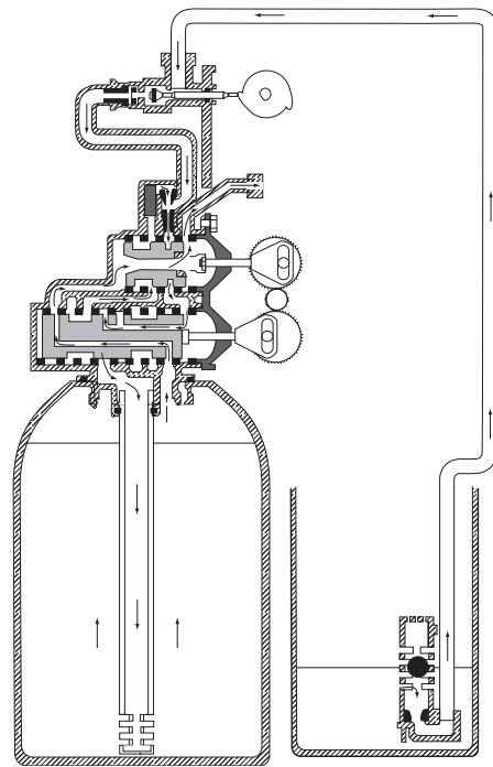
Slow Rinse Position (3)
