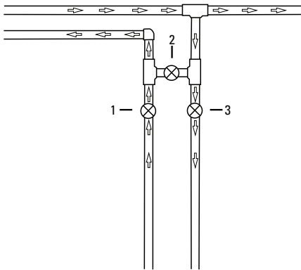
Figure 4 Manual Bypass
