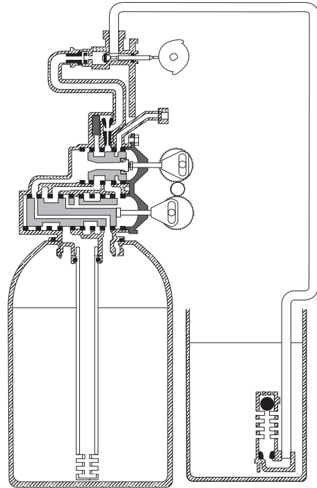
Tanks Switching Position (Meter Initiated Regeneration) (1)
